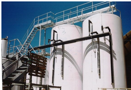
Tank and Walkway fabrication/Installation Devils Lair Winery
